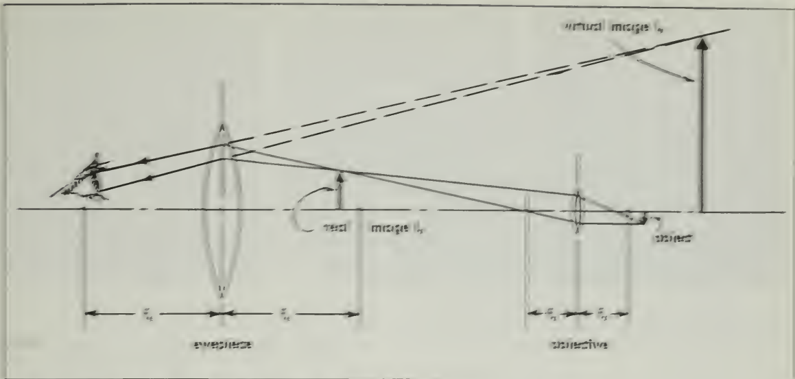
14-12. Compound microscope. The eyepiece and objective are located at the two ends of a tube. The diagram illustrates the formation of the images.
