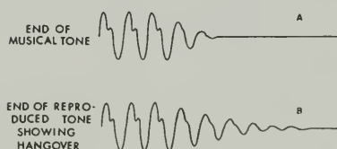
Fig. 2-3. Poor transient response.
